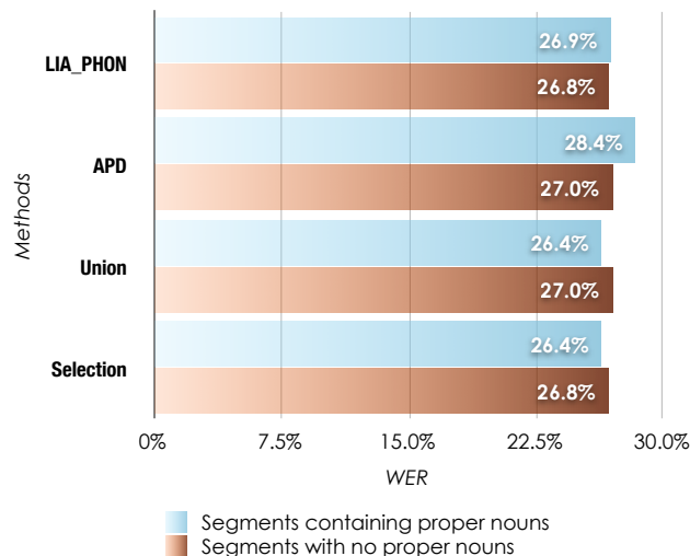
Figure 5: Word Error Rate on ESTER test corpus for segments containing proper nouns and segments with no proper nouns.
